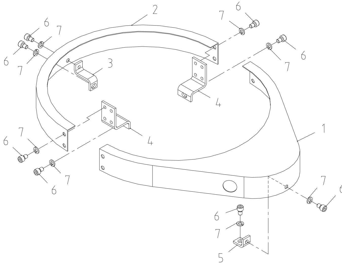
Fig. 2-1-3 SAC-2501 GEAR COVER ASS'Y
