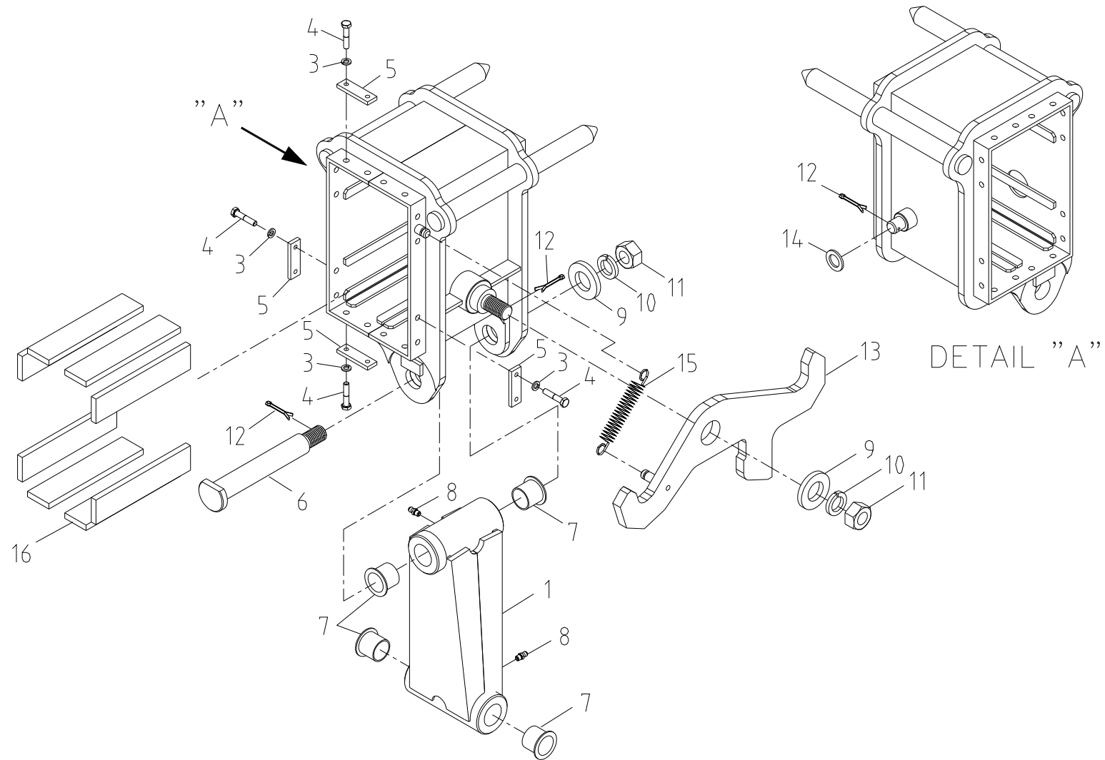
Fig. 1-1 SAC-2501 워킹 붐 조립체 WORKING BOOM ASS'Y
